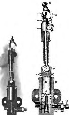
Figs. 3263-3264. Gollnar Bell Ringer. United States Metallic Packing Co.
